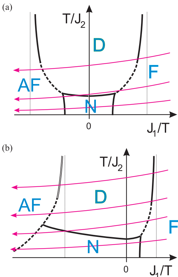
Fig. 1: (Colour on-line) Schematic structures of phase diagrams of SFS arrays with (a) bipartite lattice and (b) triangular lattice. Ferromagnetic (F), nematic (N), antiferromagnetic (AF) and disordered (D) phases are separated from each other either by continuous (continuous bold lines) or first-order (dashed bold lines) phase transitions. The double line separating AF and D phases in (b) stands for the sequence of BKT and Ising transitions with very small separation. Curved arrows going from right to left show different paths of the evolution of an array with the decrease in temperature.
